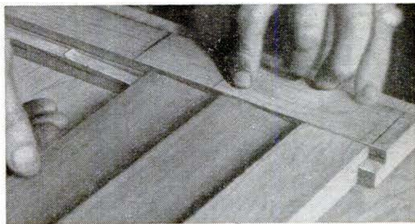
Overlap the slats slightly and glue them in position. Also glue all the joints of the frame.
